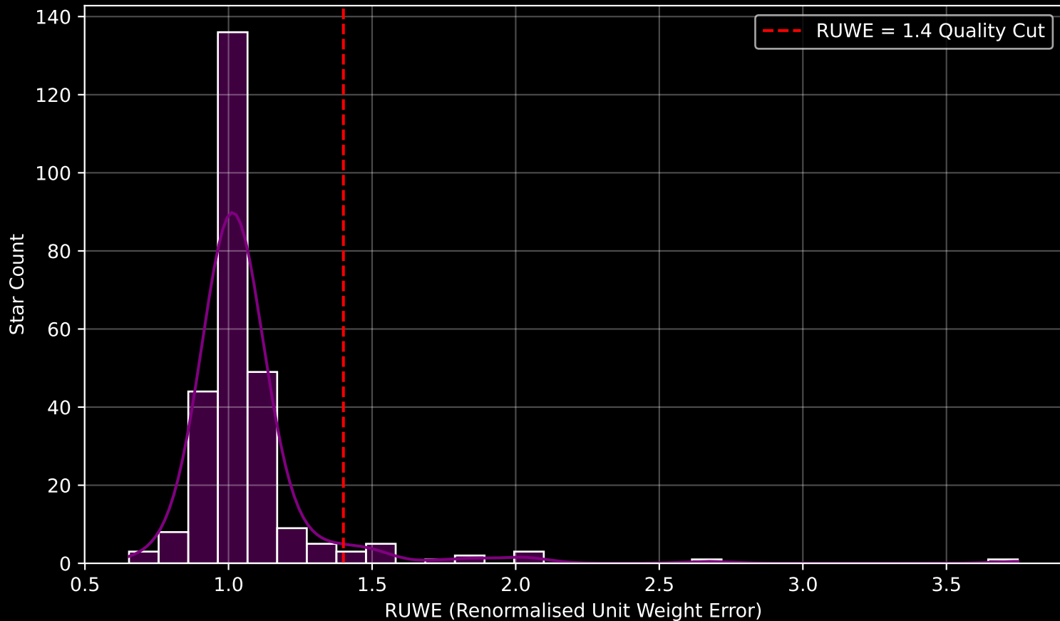
GAPOGEE DR17 Field [015-02] RUWE Distribution (n= 270)
