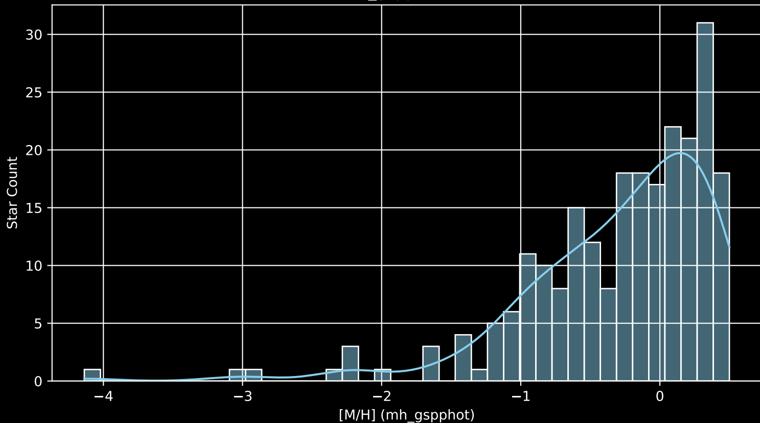
APOGEE DR17 Field: [015-02 [M/H] (mh_gspphot) (n= 236)
