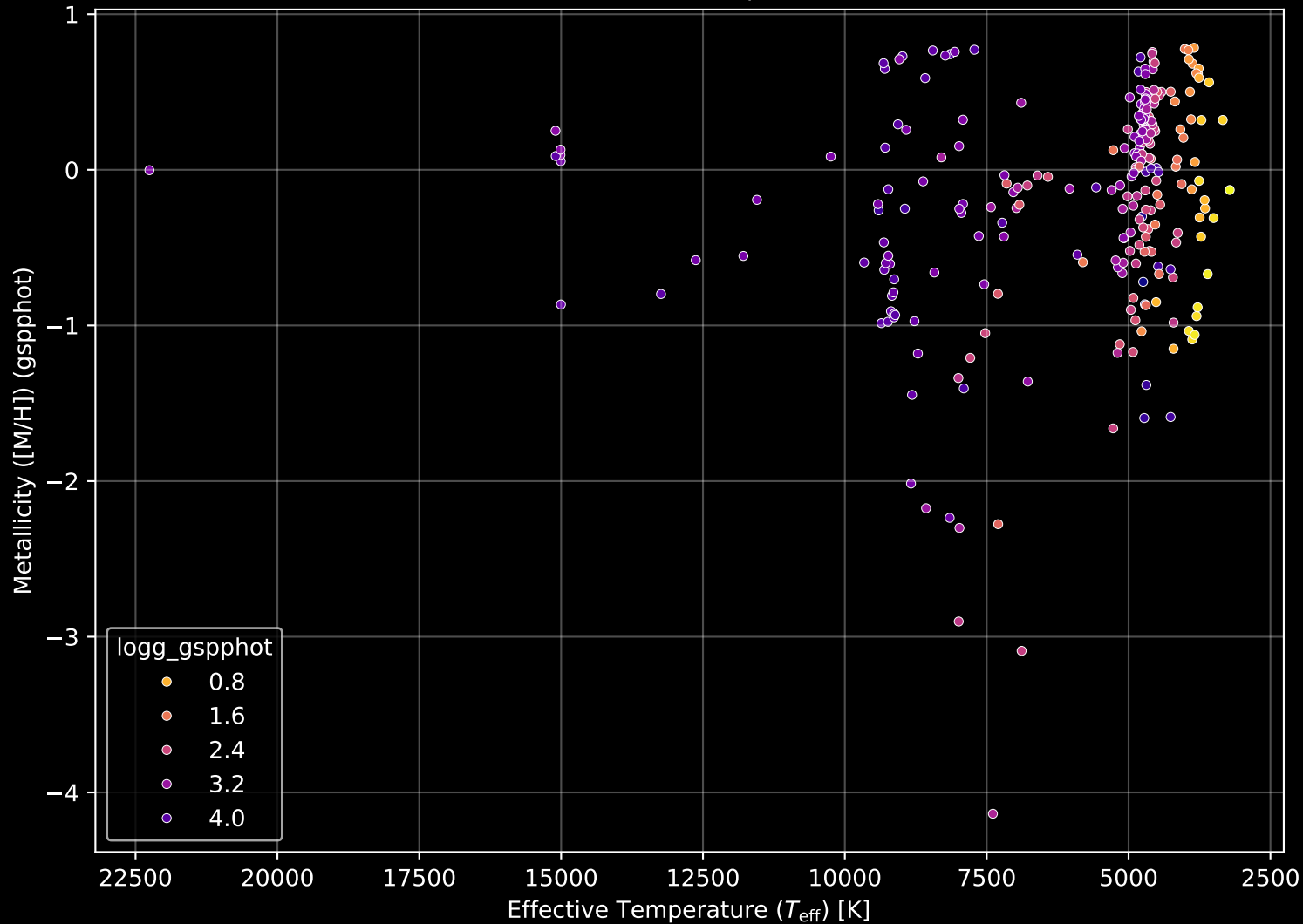
APOGEE DR17 Field: [015-02] Stellar Population Parameters (n= 271)
