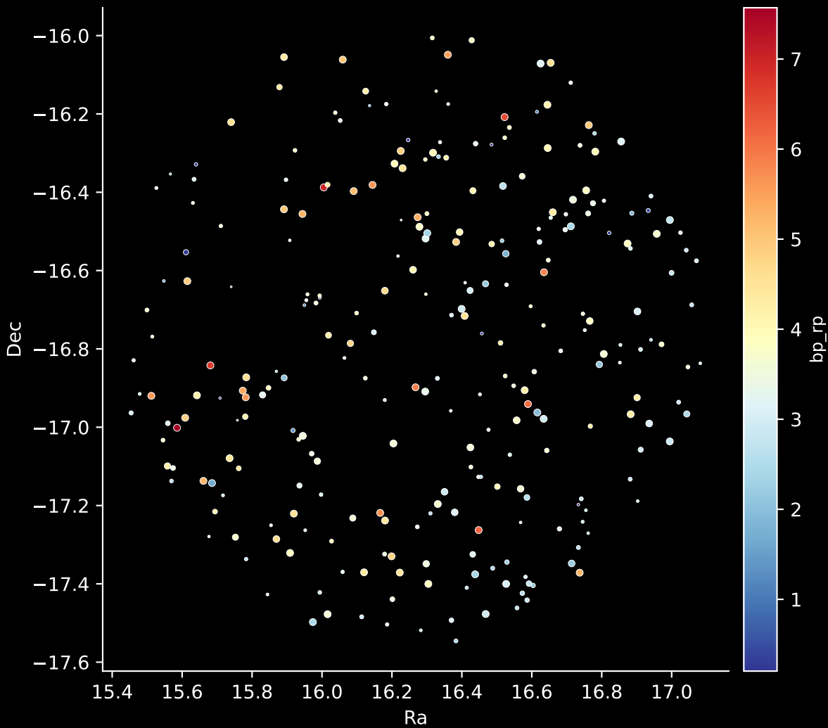
APOGEE DR17 Field: [015-02] Stars: 271
