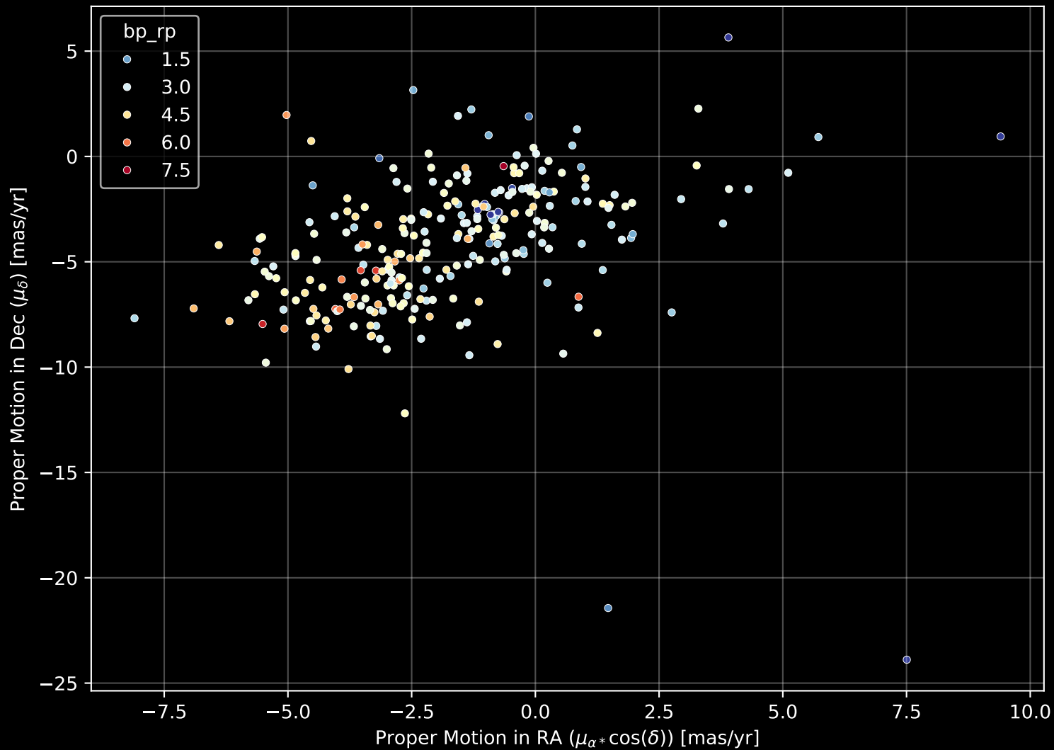
APOGEE DR17 Field: [015-02] Proper Motion Diagram (n= 271)
