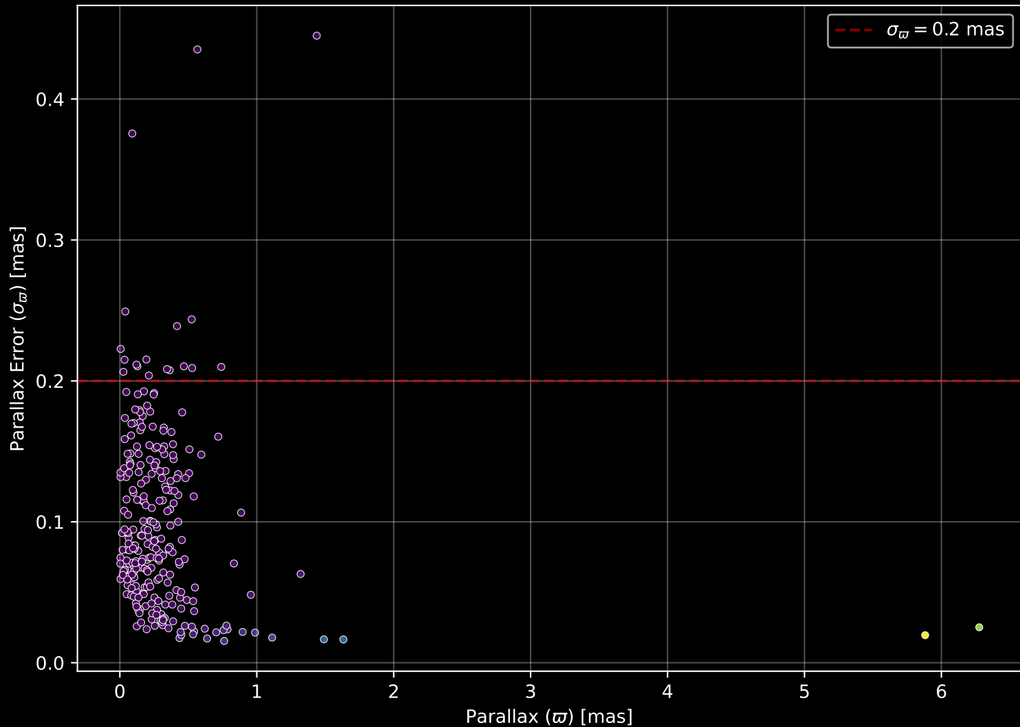
APOGEE DR17 Field: [015-02] Parallax Quality (n= 271)
